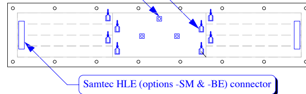
FEE Board, Top Side
