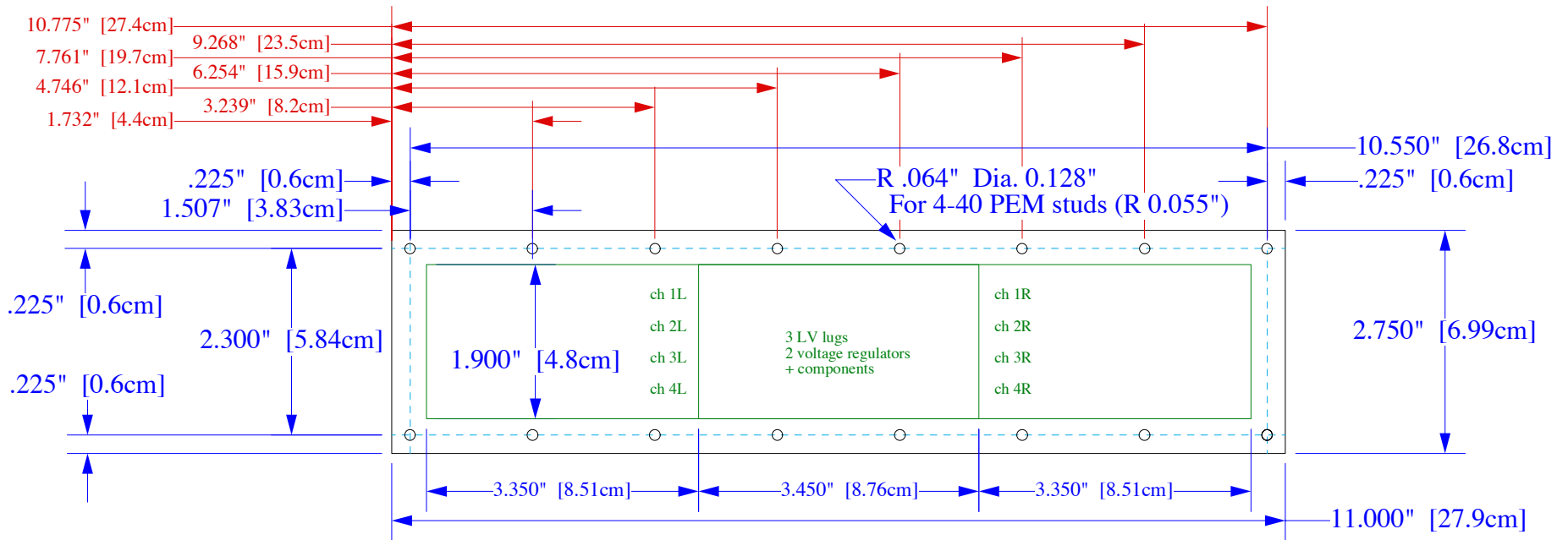
F/T Board, Bottom Side
