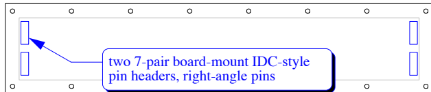
F/T Board, Bottom Side
